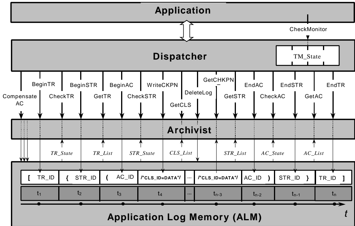
Figure. Management of the Application Log Memory by Archivist
